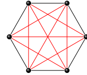
Figure 1: A hexagon has \frac{6(6-3)}{2} = 9 diagonals.
