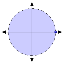
Figure 20.1: If \alpha is one of the blue points, above, then sequence \{\alpha^n\} converges. It converges to 1 if \alpha = 1 , to 0 if |\alpha| < 1 , and diverges, otherwise.
