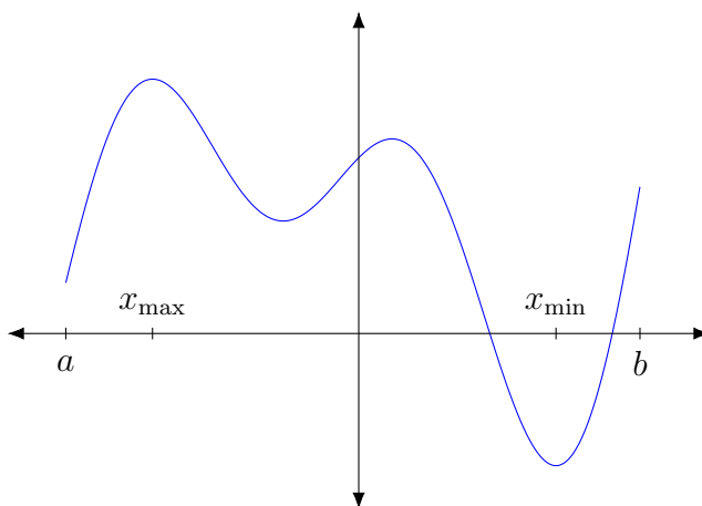
Figure 34.1: A continuous function on a closed interval [a, b] with the points at which it achieves its (global) minimum and maximum labeled.
