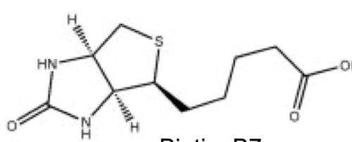
Biotin, B7
