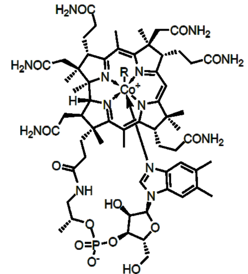
Cobalamin, B12
