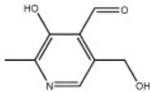
Pyridoxal, B6
